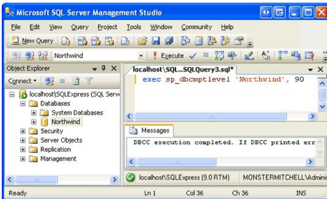
Figure 9: Update the Northwind Database’s Compatibility Level
